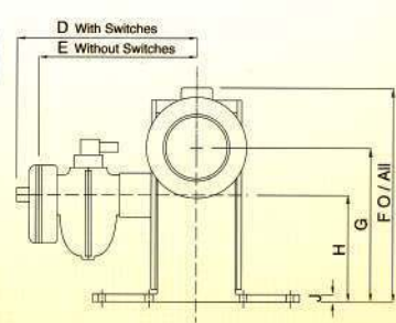
Mounting Flange Detail
